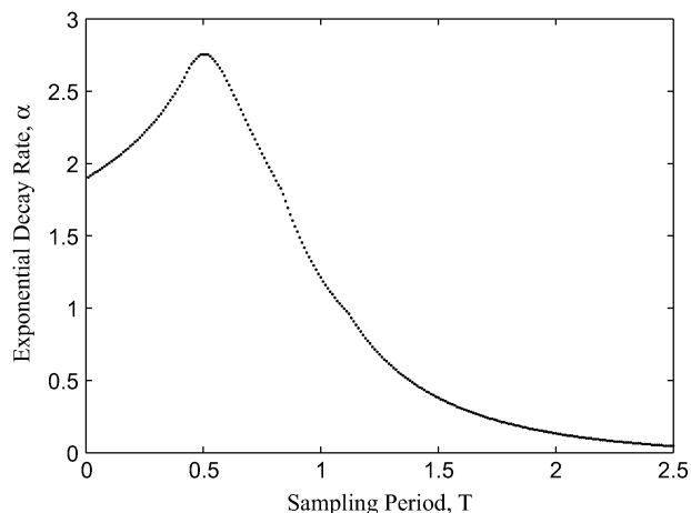
Fig. 1. Bound on decay rate vs. asynchronous sampling period, T_{\max} and T_{\min} = 0.9T_{\max} for Example 2 with N = 3 .
