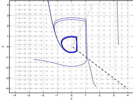
Fig. 9. Trajectories of Hybrid System in Example 5 with p=0.4 . Dotted line indicates G_{12} and dash-dotted line indicates G_{21}
