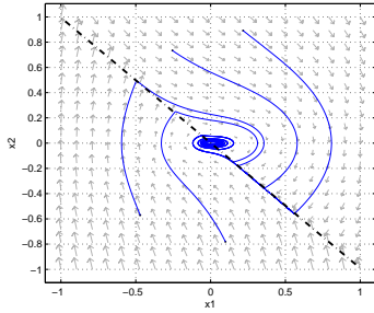
Fig. 5. Hybrid system of Example 2. The dashed line indicates x_2 + x_1 = 0 .
