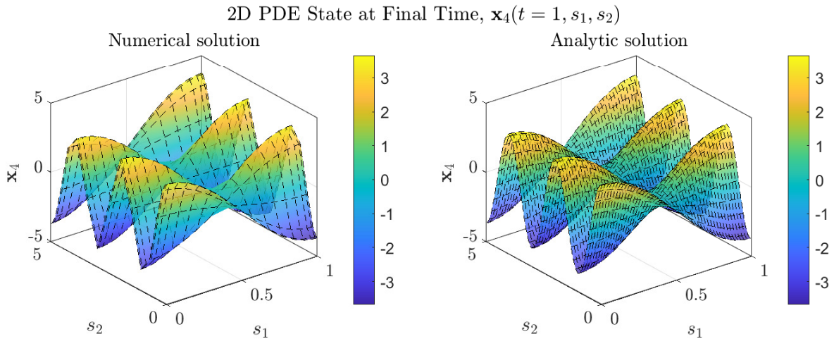
Figure 6.3: Numerical and true values of the 2D PDE state \mathbf{x}_4(t) from the ODE-PDE (6.2) at t = 1 , simulated with initial conditions as in (6.3).
