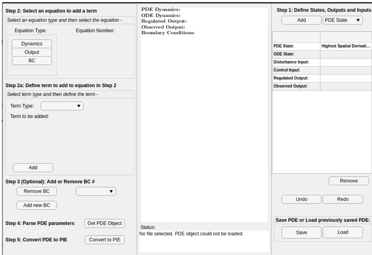
Figure 4.1: Example of empty GUI window.
