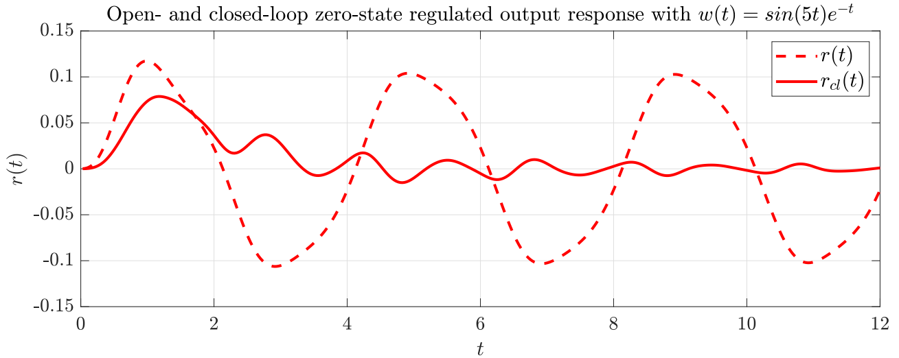
Figure 2.3: Open- ( r(t) ) and closed-loop ( r_{cl}(t) ) transient response of the regulated output r(t) for external disturbance w(t) = \sin(5t)e^{-t} .
