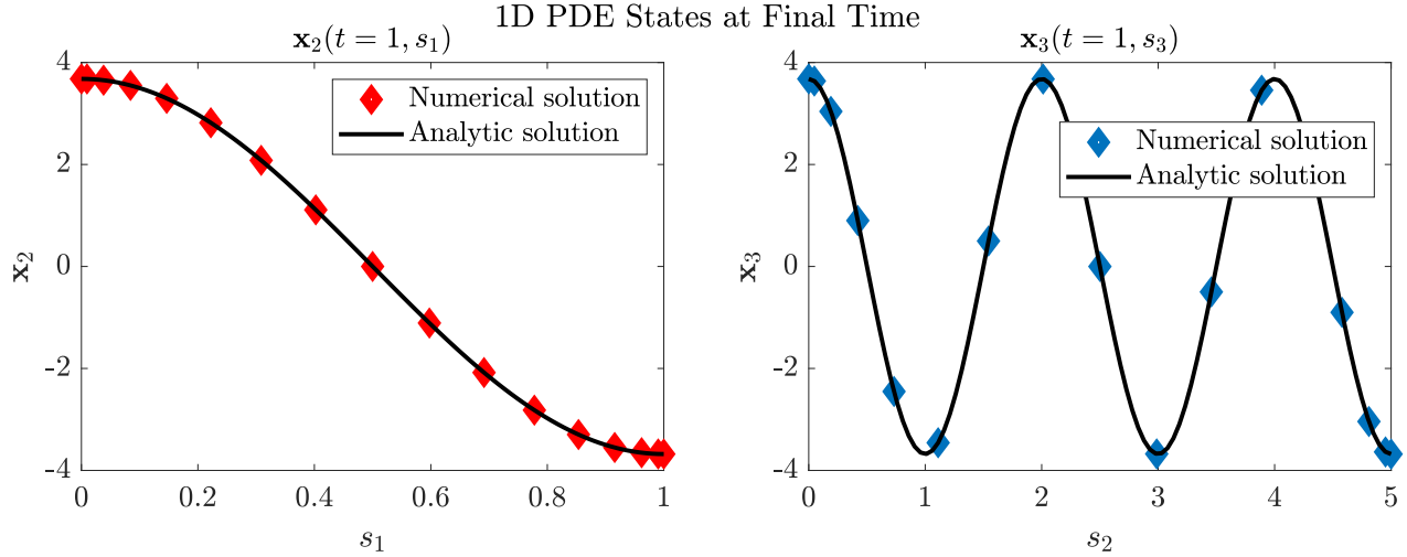
Figure 6.2: Numerical and true values of the 1D PDE states \mathbf{x}_2(t) and \mathbf{x}_3(t) from the ODE-PDE (6.2) at t = 1 , simulated with initial conditions as in (6.3).
